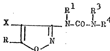
(I-i: R 4 =Alkylmercaptorest)
